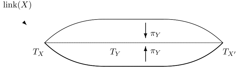
Figure 2: Tubular neighborhoods
